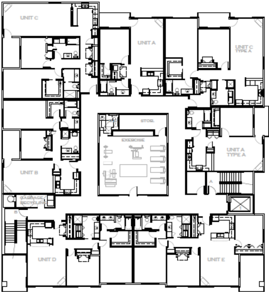
SOUTH BUILDING FLOOR PLAN
